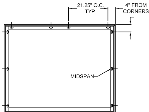
TYPICAL ELEVATION WITH FASTENER SPACING
